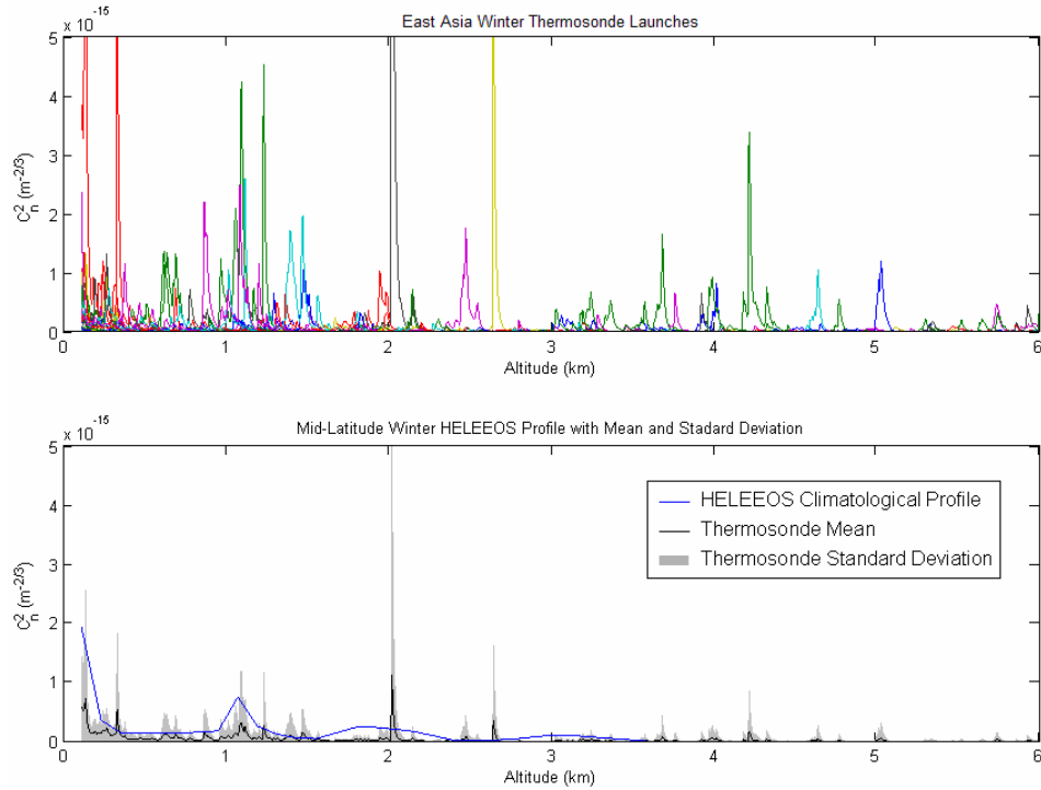
Figure 29: Comparison of the East Asia winter thermosonde data to the corresponding HELEEOS correlated optical turbulence climatology. The top plot is each raw thermosonde profile, and the bottom contains the comparison between the HELEEOS correlated C_n^2 climatology and the thermosonde data mean and standard deviation. The boundary layer height for this scenario is 500 m.
