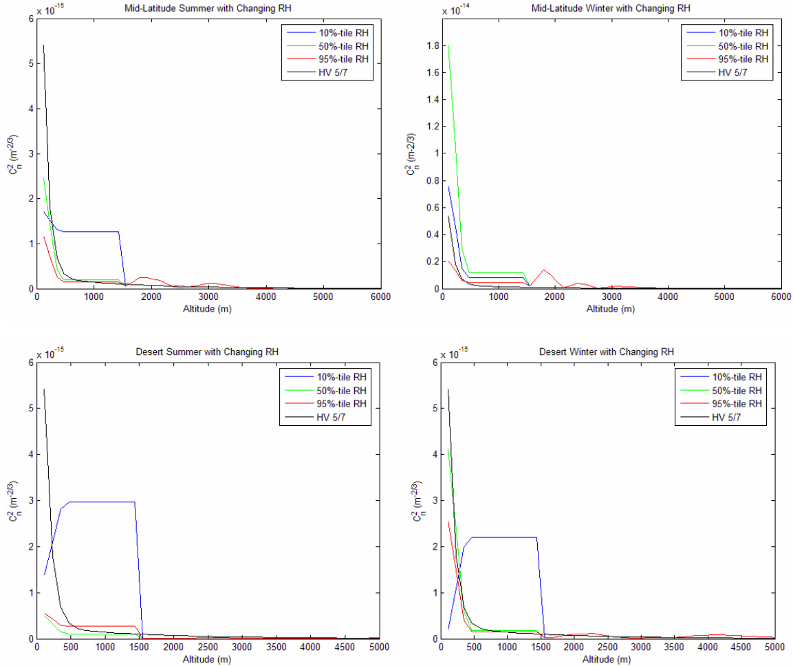
Figure 17: Mid-Latitude and desert summer and winter optical turbulence profiles for 10 th percentile, 50 th percentile, and 95 th percentile relative humidity plotted against Hufnagel-Valley 5/7.
